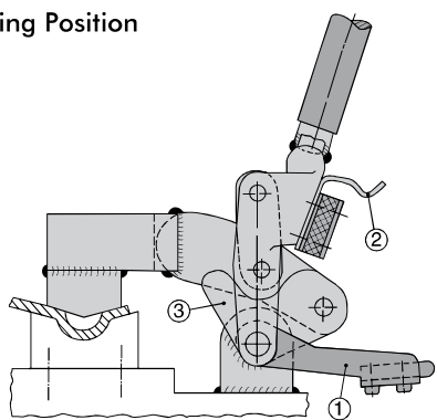
Clamping Position
