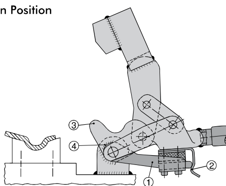
Open Position
